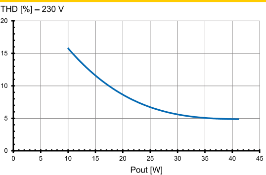
Total harmonic factor (THD) at 230 V
