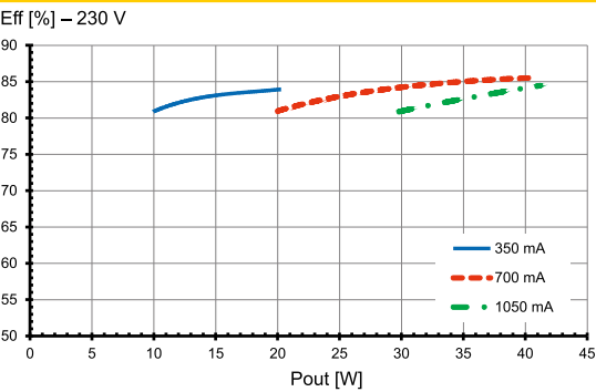
Efficiency at 230 V
