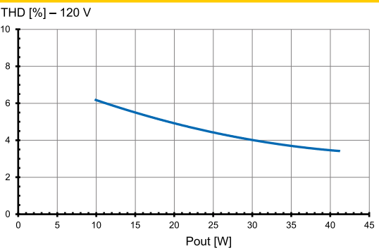
Total harmonic factor (THD) at 120 V
