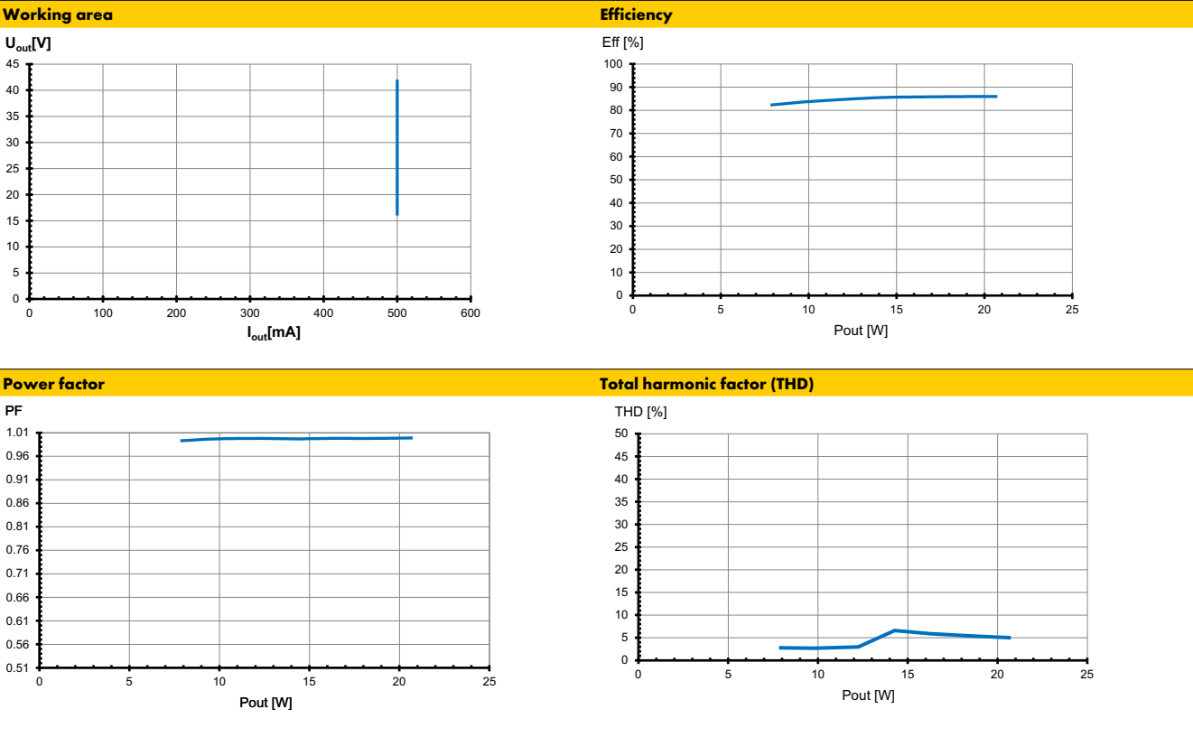
Typ. performance graphs for 187607 / Type ECXd 500.750 at 100 V
