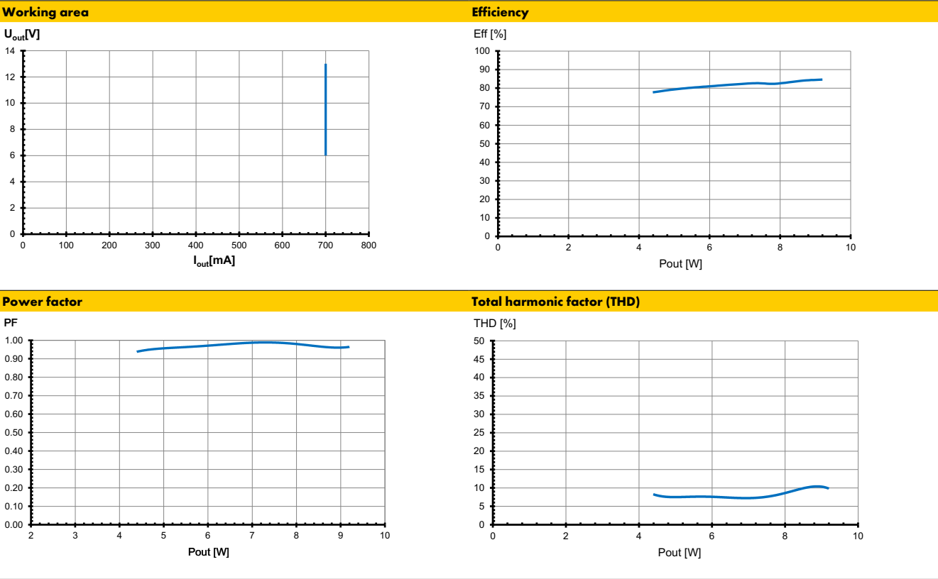
Typ. performance graphs for 187605 / Type ECXd 700.748 at 100 V
