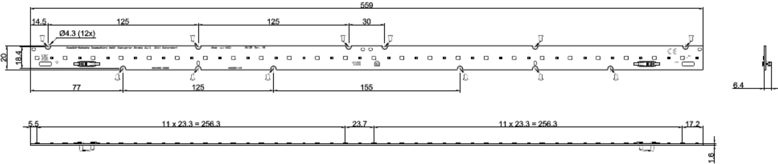
MLC SC W2/560 B/24R/xxx G3
