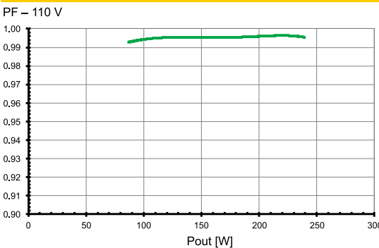
Power factor at 110 V
