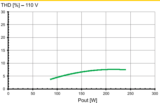
Total harmonic factor (THD) at 110 V
