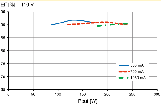
Efficiency at 110 V
