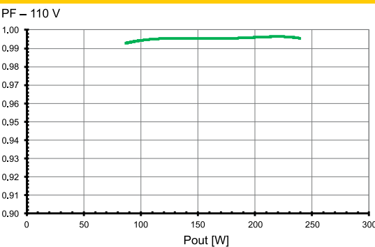
Power factor at 110 V
