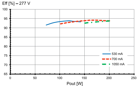
Efficiency at 277 V
